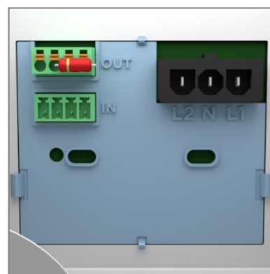
Install Terminating Resistor
